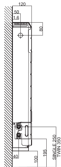
SIDE VIEW TYPE 100
