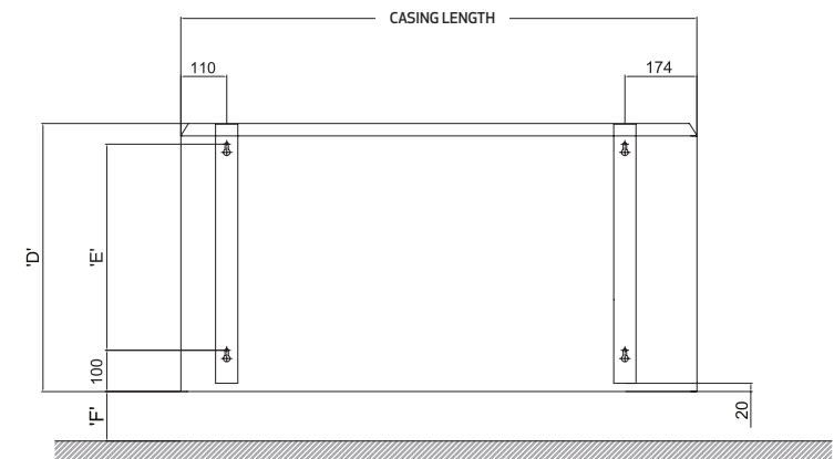
FRONT VIEW - RIGHT HAND VALVE POSITION BRACKET FIXING DETAIL
