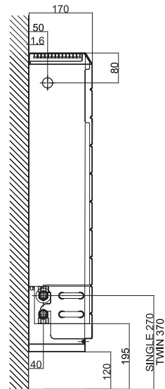
SIDE VIEW TYPE 150
