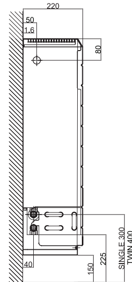
SIDE VIEW TYPE 200
