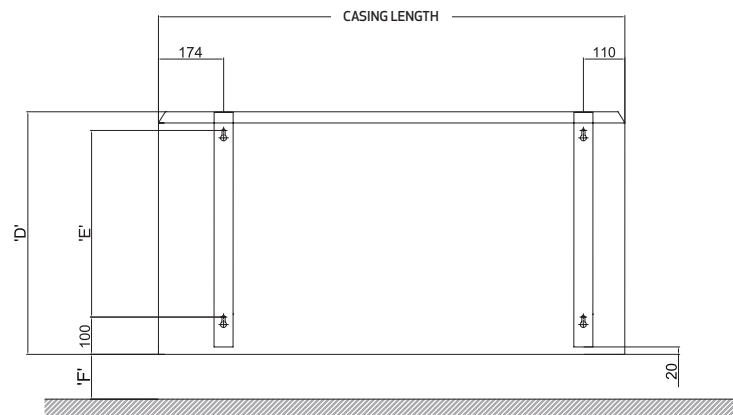
FRONT VIEW - LEFT HAND VALVE POSITION BRACKET FIXING DETAIL
