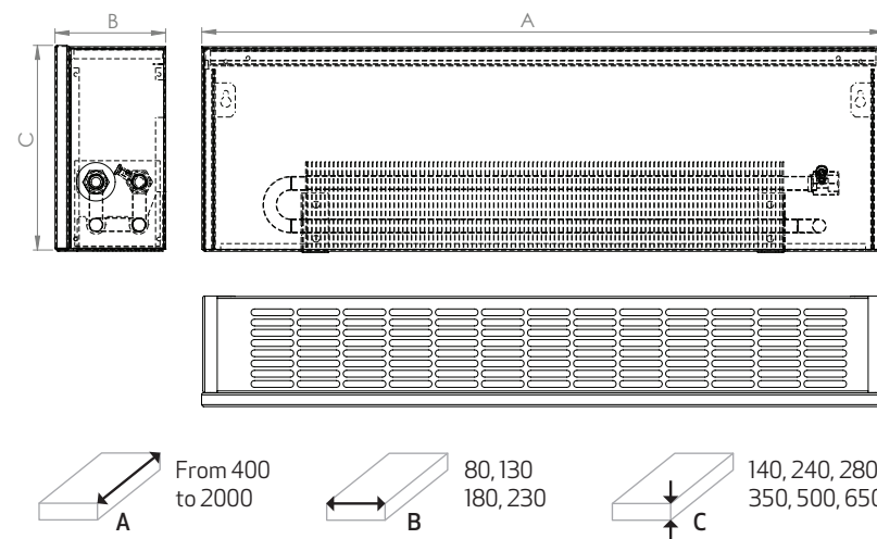
Dimensions (mm)
